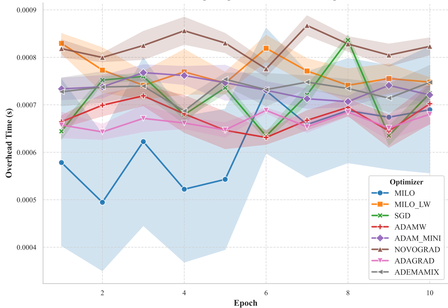
Overhead Runtime per Epoch for LOGISTIC Experiment
